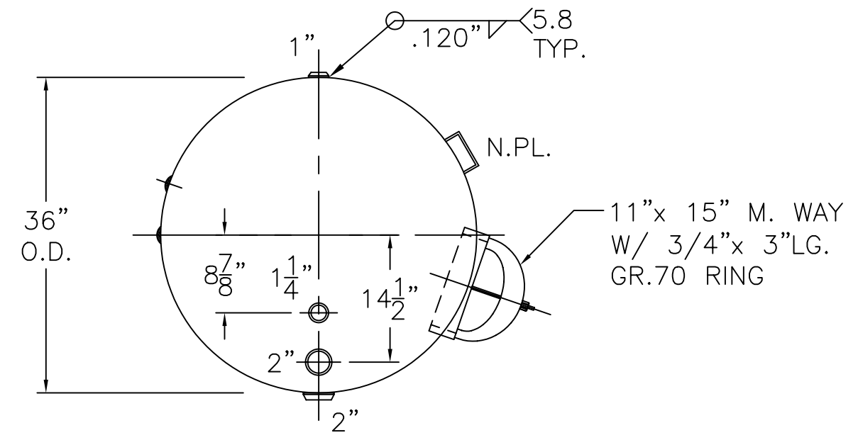
END VIEW W/OUT SUPPORTS
